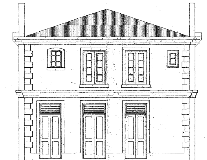
EAST ELEVATION
